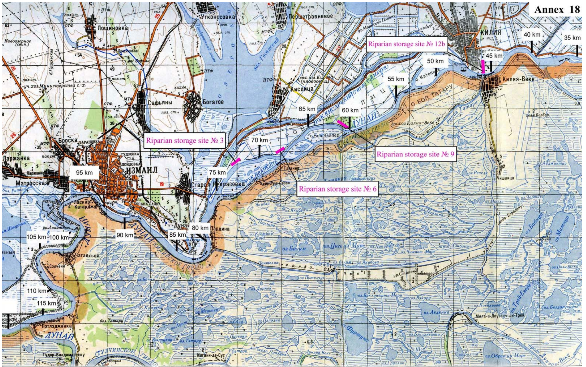
Disposition of riparian storage sites along Deep Water Navigation Route
